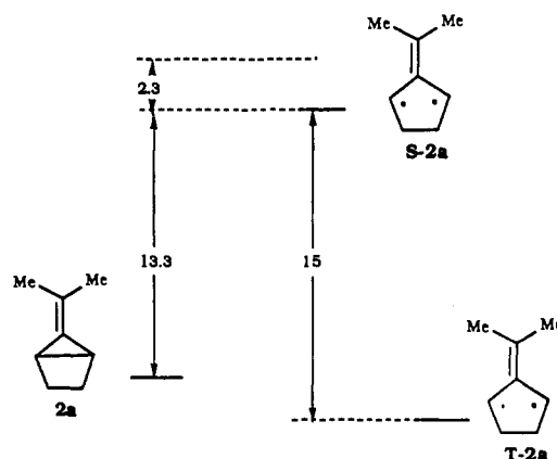
Figure 1. Energy diagram for the non-Kekulé diradicals S-2a and T-2a .
