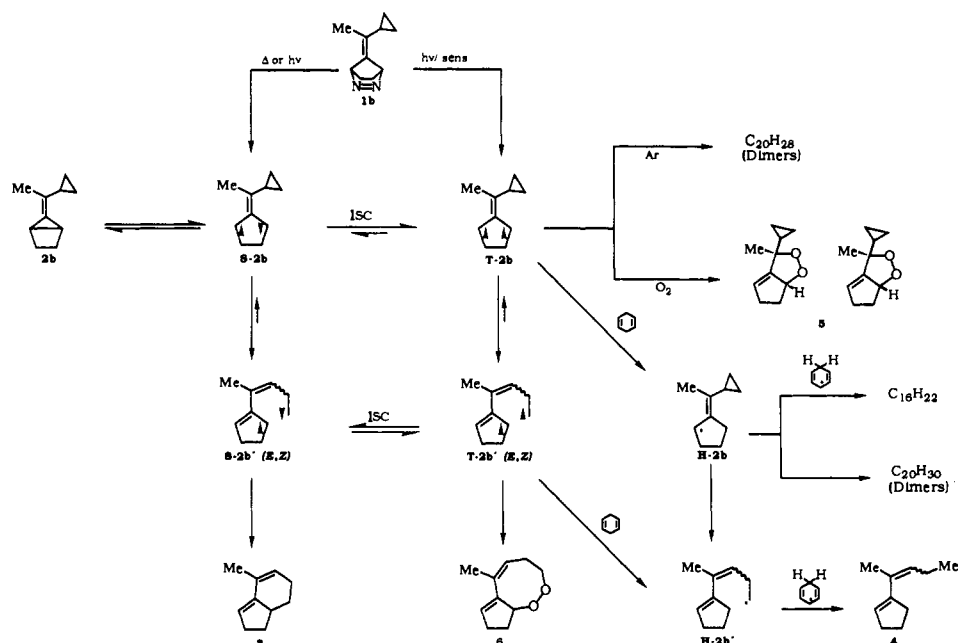
Scheme I. Products and Reaction Pathways of the Singlet (S-2b) and Triplet Diradicals (T-2b)
